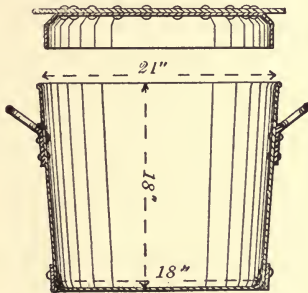
FIG. 1.—MODIFIED BIRMINGHAM PAI L .
